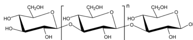
Fig. 6. Chemical structure of curdlan.
