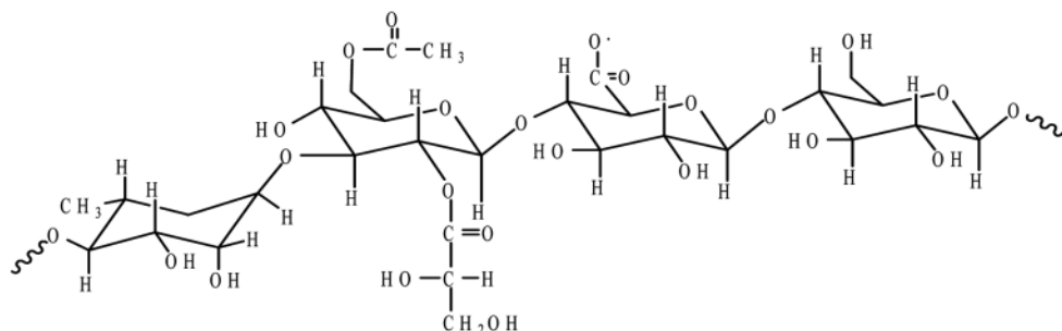
Fig. 5. Chemical structure of gellan.
