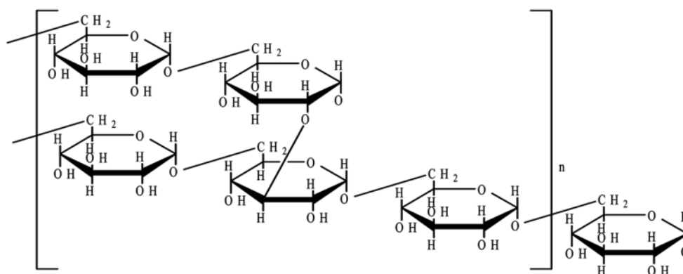
Fig. 1. Chemical structure of dextran.
